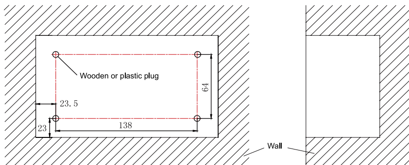
Figure 3-10 Diagram of Wooden or Plastic Plug
