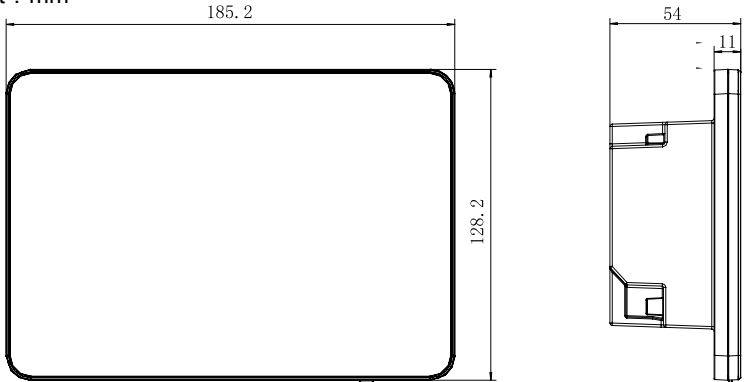
Figure 3-2 Dimension of Centralized Controller
